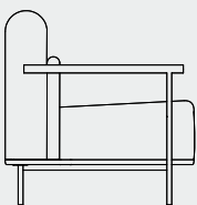
MBRM1B W 720 mm H 730 mm D 730 mm S 420 mm 26,9 Kg
